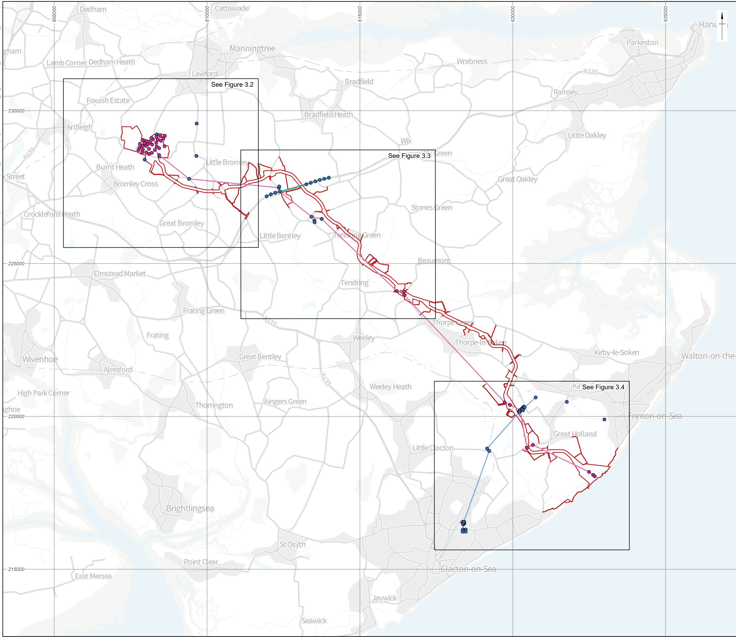
Figure 3.1: Location of BGS archive boreholes and recent geoarchaeological works, showing Transects A-C
