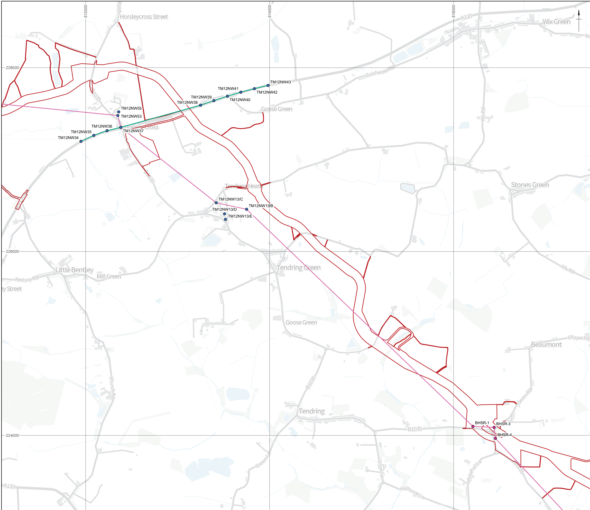
Figure 3.3: Location of BGS archive boreholes and recent geoarchaeological works, showing Transects A-C
